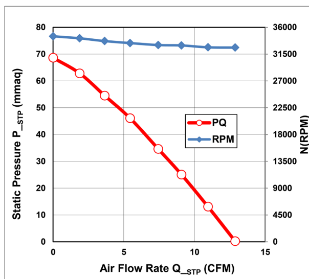
Back to Front Airflow (HB4C) Model
