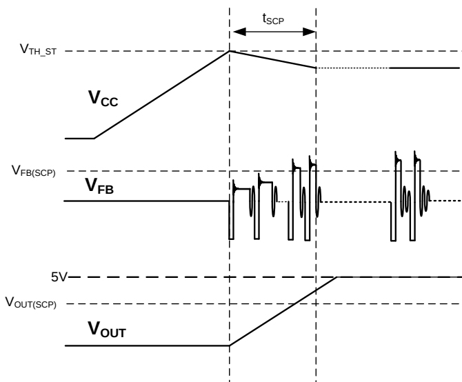
Figure 6 Normal Start-up
