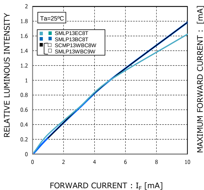
Fig.3 Luminous Intensity - Forward Current
