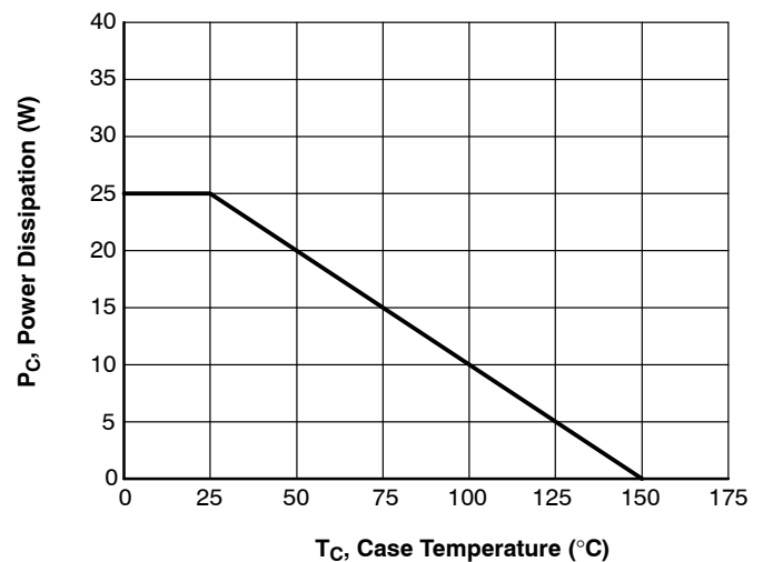
Figure 6. Power Derating
