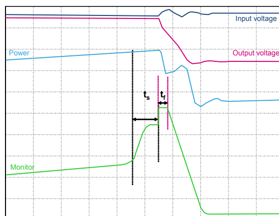
Figure 19. Monitor signal vs. power (zoom)
