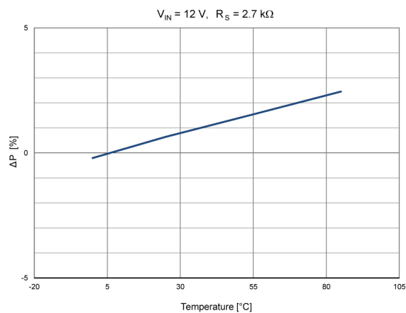
Figure 14. Power limit accuracy vs. temperature
