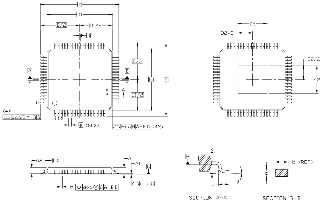
Figure 39. 64-Pin Thin Quad Flat Package (TQFP)
