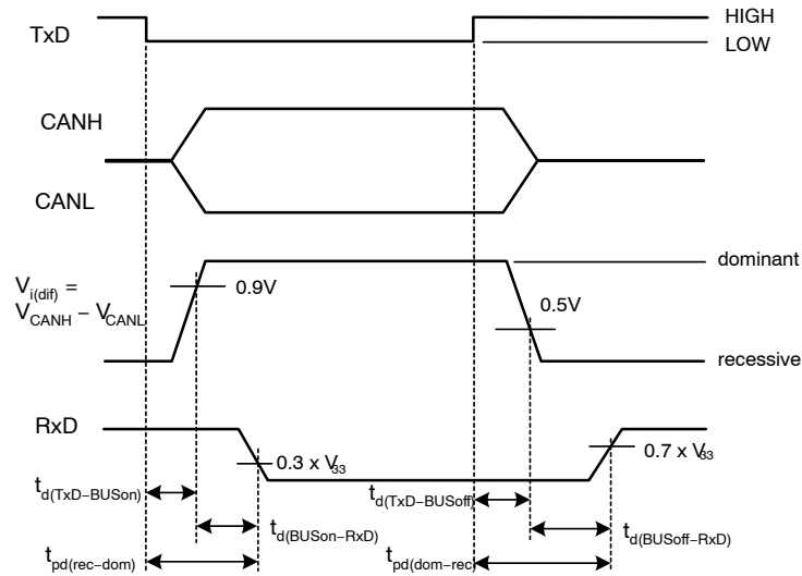
Figure 6. Timing Diagram for AC Characteristics
