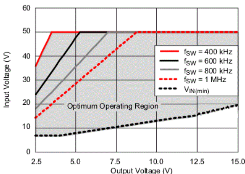
Figure 27. Optimum Operating Range with Switching Frequency
