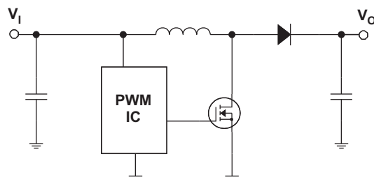
Figure 16. Typical Boost Converter Topology
