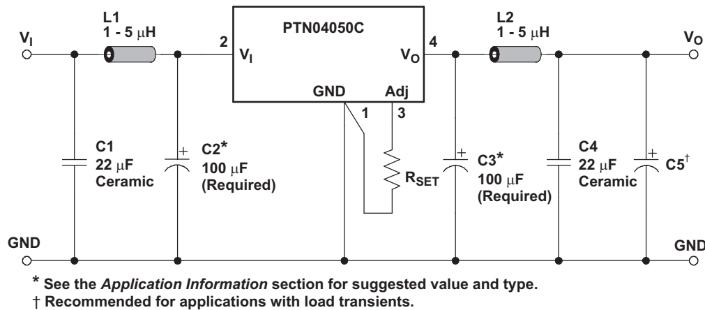
Figure 18. Adding π Filters
