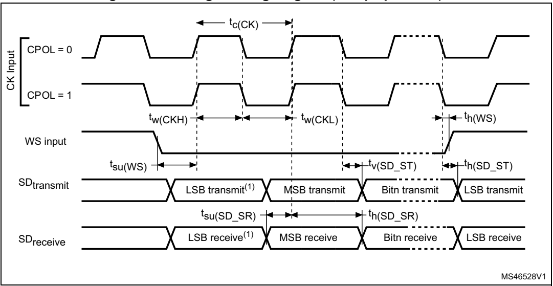
Figure 49. I 2 S target timing diagram (Philips protocol) (1)
