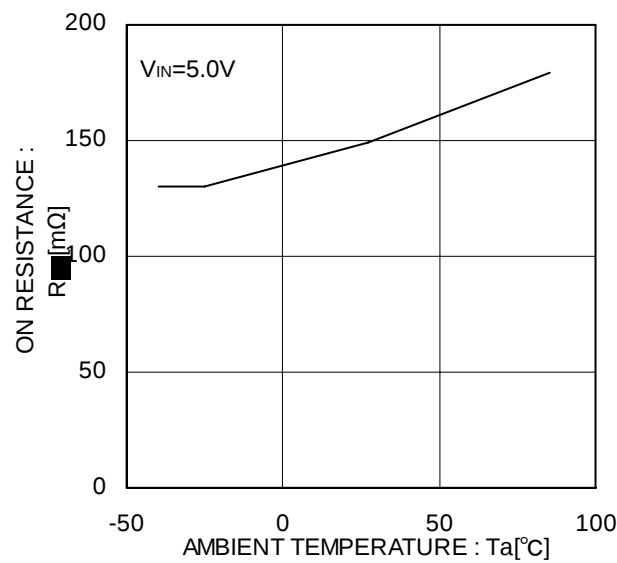
Figure 10. ON resistance
