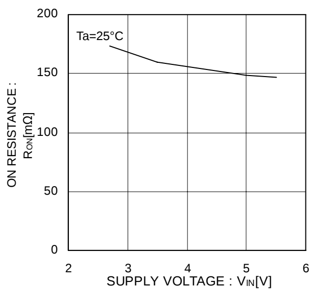
Figure 9. ON resistance
