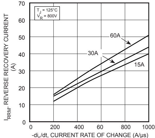
FIGURE 28, Reverse Recovery Current vs. Current Rate of Change
