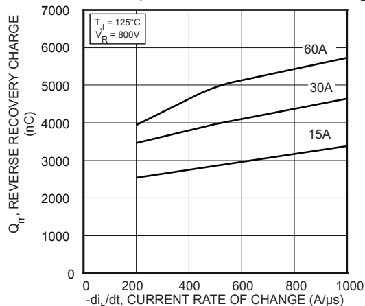
FIGURE 27, Reverse Recovery Charge vs. Current Rate of Change
