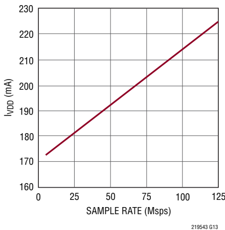
LTC2195: I_{VDD} vs Sample Rate, 5MHz, -1dBFS Sine Wave Input
