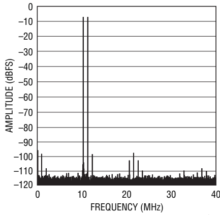
LTC2193: 64k Point, 2-Tone FFT, f_{IN} = 69\text{MHz} , 70\text{MHz} , -7\text{dBFS} , 80\text{Msps}
