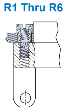
Jackpost for Rear Panel Mounting Shipped loosely installed. Install with permanent threadlocking compound.
