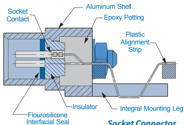
Socket Connector
