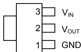
Tab is V_{OUT} SOT89-3L
