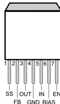
KTW Package 7-Pin DDPAK Top View
