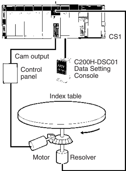
C200H-CP114 Cam Positioner Unit
