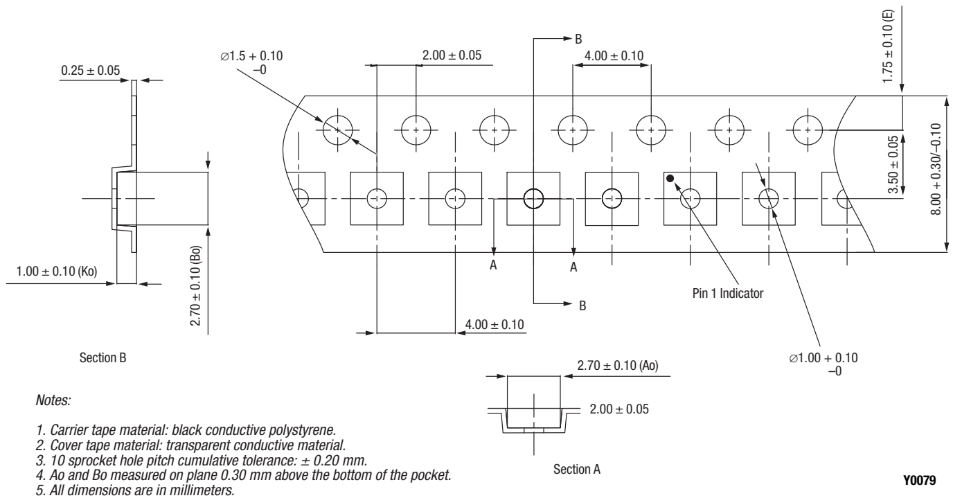
Figure 13. SKY13473-569LF Tape and Reel Dimensions
