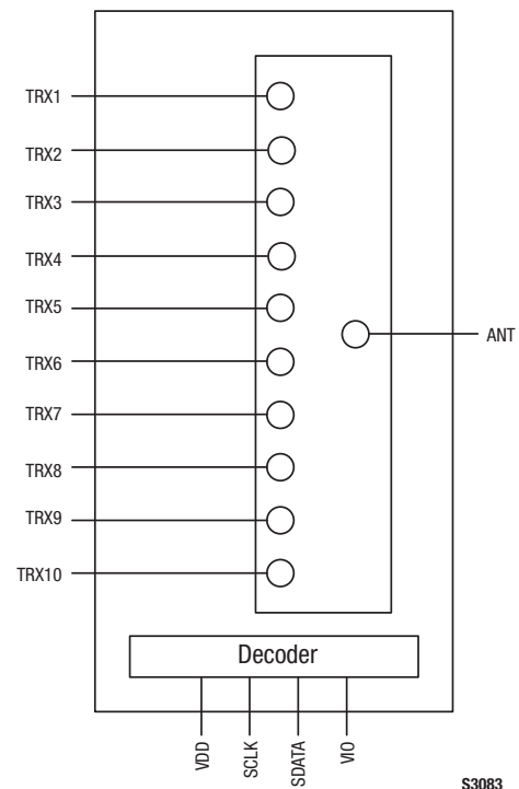
Figure 1. SKY13473–569LF Block Diagram
