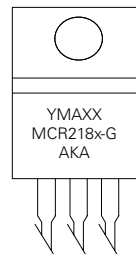
TO-220AM Case 221A Style 12
