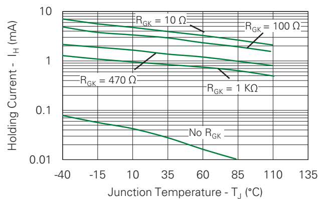
Fig. 13-2. Typical DC Holding Current with R_{GK} vs. Junction Temperature for EC103x1
