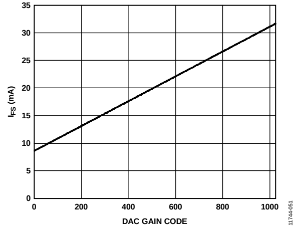
Figure 46. DAC Full-Scale Current vs. DAC Gain Code
