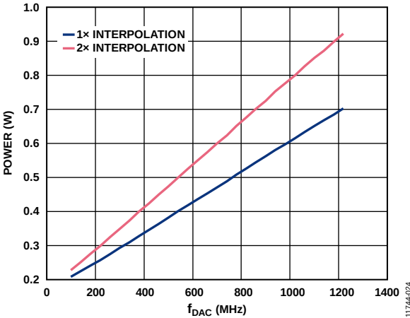
Figure 19. Total Power Consumption vs. f_{DAC} over Interpolation
