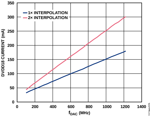
Figure 20. DVDD18 Current vs. f_{DAC} over Interpolation
