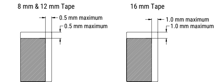
Figure 3 – Maximum Lateral Movement
