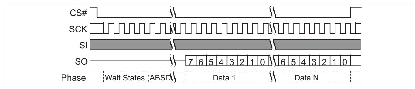
Figure 63 AutoBoot sequence (CR1[1]=0)
