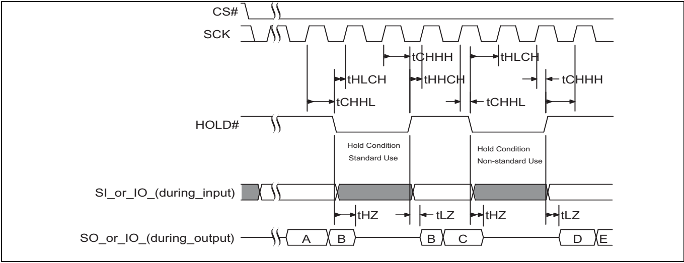
Figure 34 Hold timing
