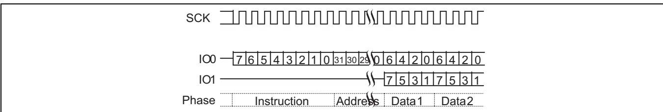
Figure 75 Dual output read command sequence (4-byte address, 3Ch or 3Bh [ExtAdd=1], LC=11b)
