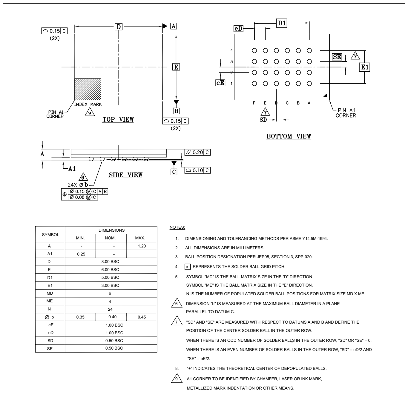
Figure 44 Ball grid array 24-ball 6x8 mm (FAC024)
