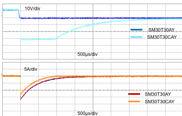
Figure 13. ISO7637-2 pulse 1 response ( V_S = -150 V) with 12 V battery
