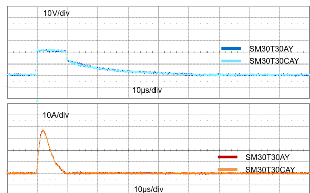
Figure 14. ISO7637-2 pulse 2a response ( V_S = 112 V) with 12 V battery
