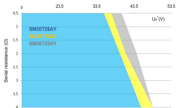
Figure 22. Load dump capability ( U_s^* = f(R_i) test B, U_s = 87\text{ V} , t_p = 400\text{ ms} )
