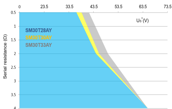
Figure 21. Load dump capability ( U_s^* = f(R_i) test B, U_s = 87\text{ V} , t_p = 150\text{ ms} )
