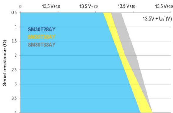
Figure 19. Load dump capability ( U_S^* = f(R_i) pulse 5b, U_S = 87\text{ V} , t_p = 400\text{ ms} )
