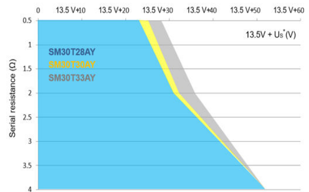
Figure 18. Load dump capability ( U_S^* = f(R_i) pulse 5b, U_S = 87\text{ V} , t_p = 150\text{ ms} )
