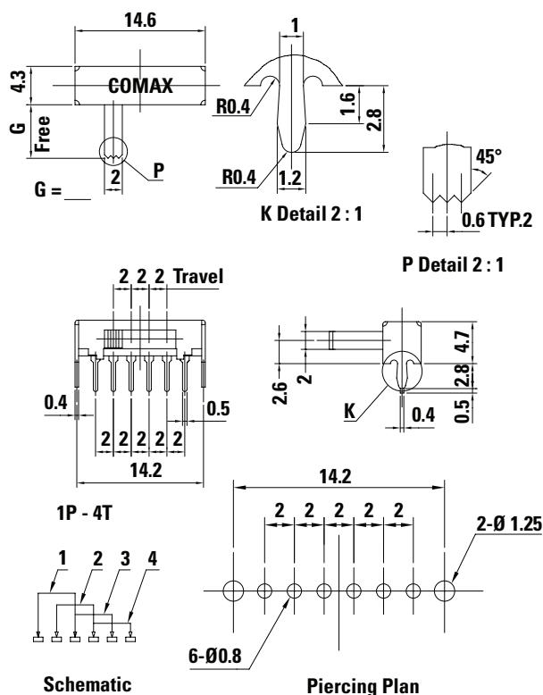
SK-14D01-G 6 1P4T 6mm Knob
