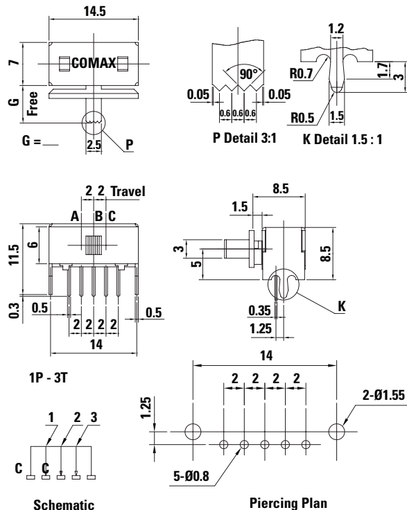
SK-13D37-G 6 NS 1P3T Non-Shorting 6mm Knob
