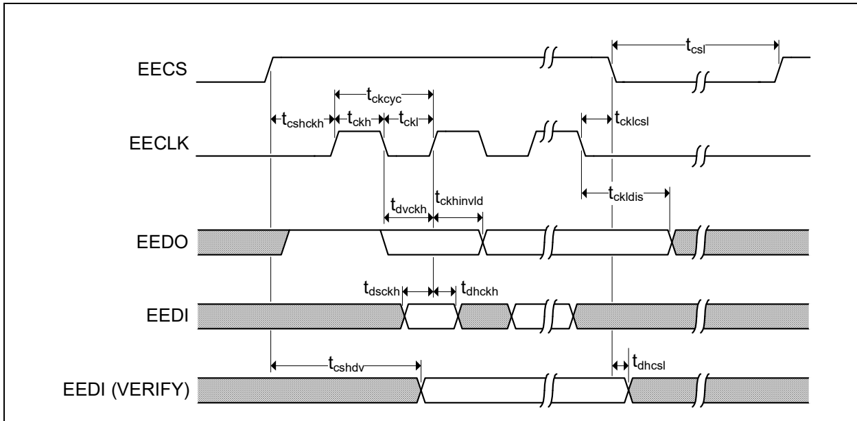
FIGURE 16-4: EEPROM TIMING
