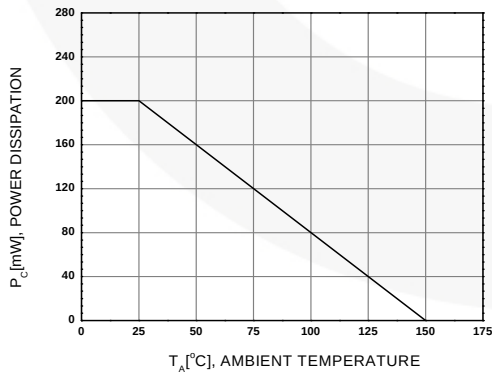
Figure 5. Power Derating
