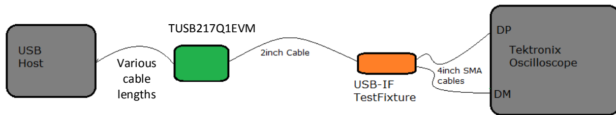
Figure 8. Near End Eye Measurement Set up With Pre-channel Cable
