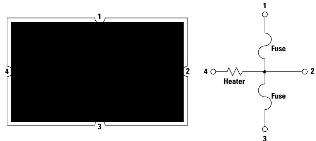
Device Circuit
