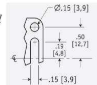
bracket detail
