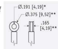
eyelet detail
