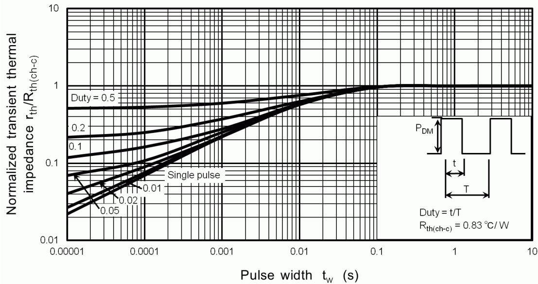
Fig. 8.15 r_{th}/R_{th(ch-c)} - t_w (Guaranteed Maximum)
