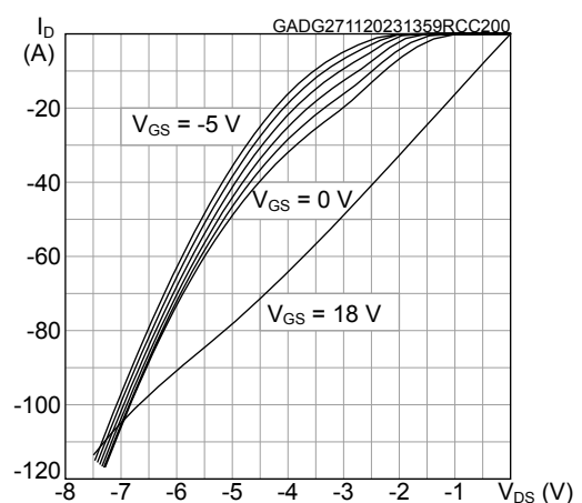
Figure 18. Typical reverse conduction characteristics ( T_J = 200^{\circ}\text{C} )
