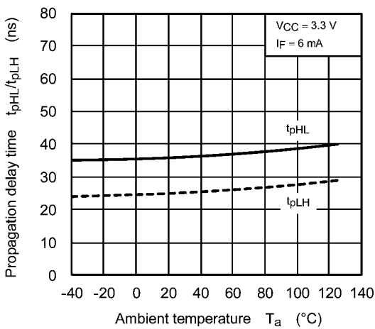
Fig. 12.2.9 t_{pHL}/t_{pLH} - T_a
