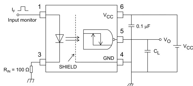
Fig. 12.1.5 Switching Time Test Circuit and Waveform
