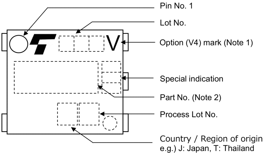
Fig. 16.4 Marking Example
