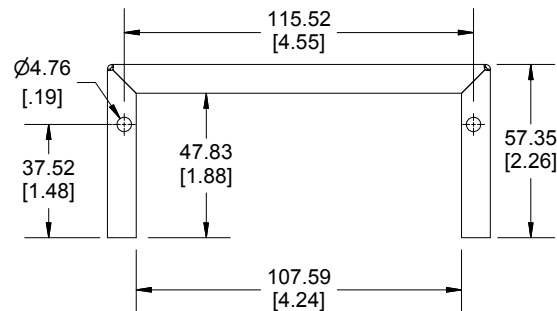
Side View of Cover
