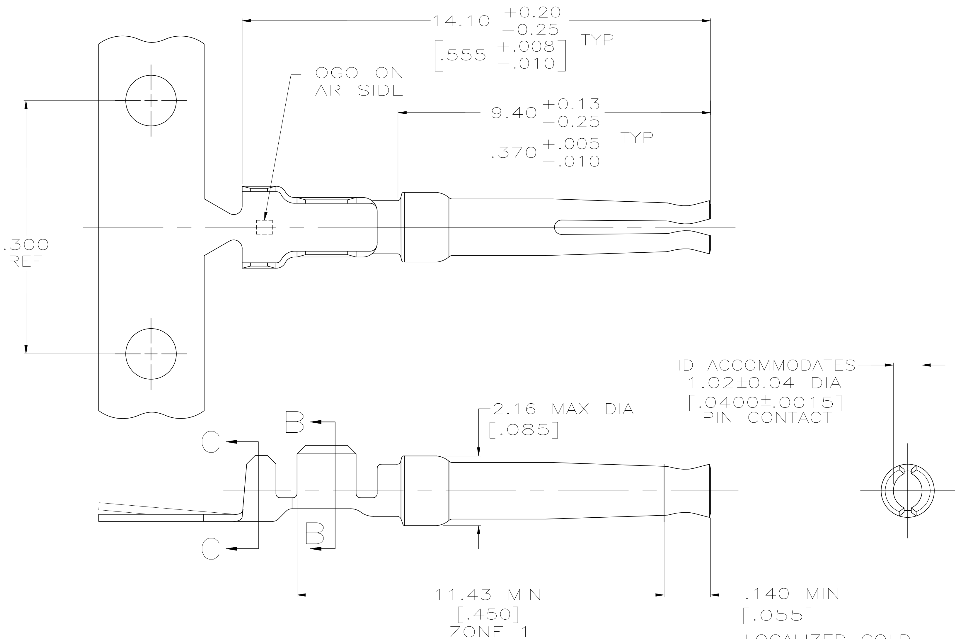
DETAIL Z SCALE 8:1
