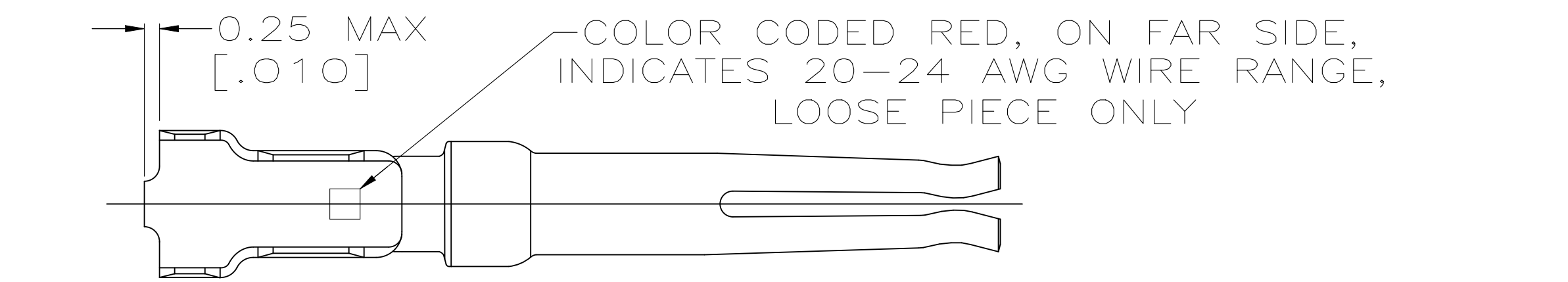
DETAIL Z SCALE 8:1
