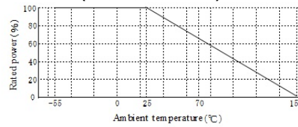
■ PML100(1.0,1.5,2.0,2.2mΩ)
