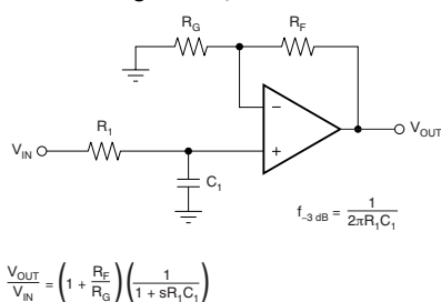
Single-Pole, Low-Pass Filter
