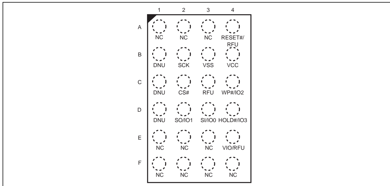
Figure 4 24-ball BGA, 4 × 6 ball footprint (FAC024), top view [9]
