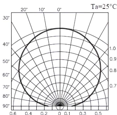
Radiation Diagram
