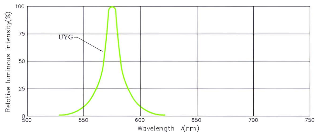
Spectrum Distribution
