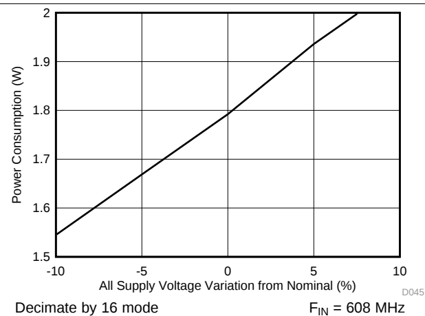
Figure 13. Power Consumption vs Supply
