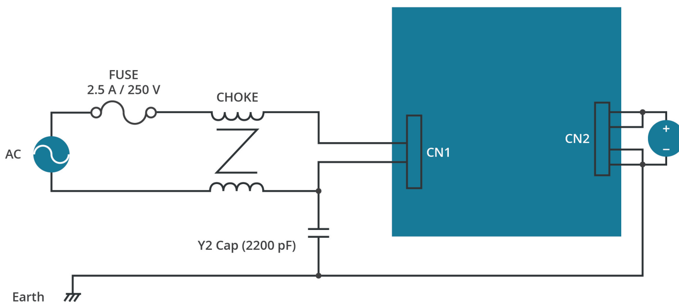
Figure 4 Board mount
