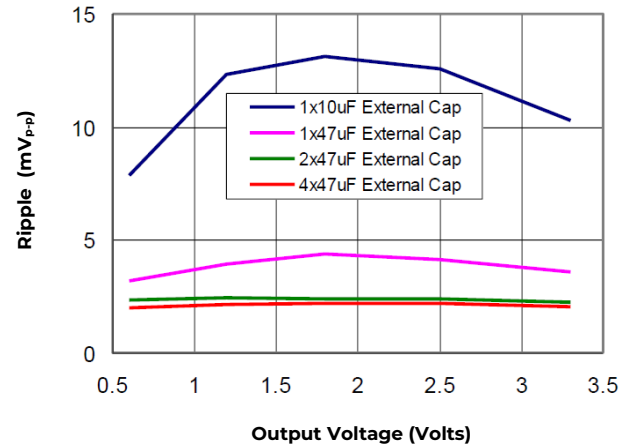
Figure 36. Output ripple voltage for various output voltages with external 1x10 µF, 1x47 µF, 2x47 µF or 4x47 µF ceramic capacitors at the output (12A load). Input voltage is 5V.
