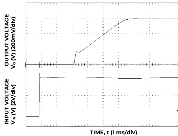
Figure 6. Typical Start-up Using Input Voltage (V IN = 5 V I o = I o, max .)
