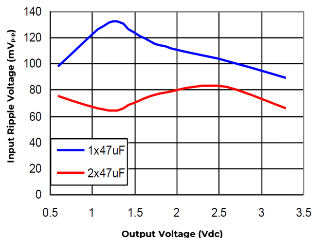
Figure 34. Input ripple voltage for various output voltages with 1 \times 47\mu F or 2 \times 47\mu F ceramic capacitors at the input (12A load). Input voltage is 5V.
