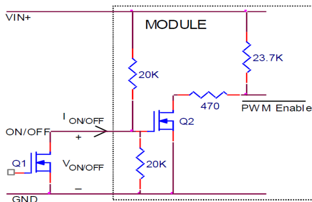
Figure 38. Circuit configuration for using positive On/Off logic.
