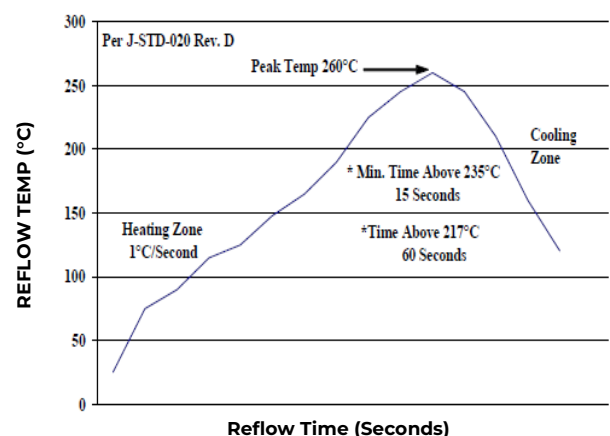
Figure 47. Recommended linear reflow profile using Sn/Ag/Cu solder.
