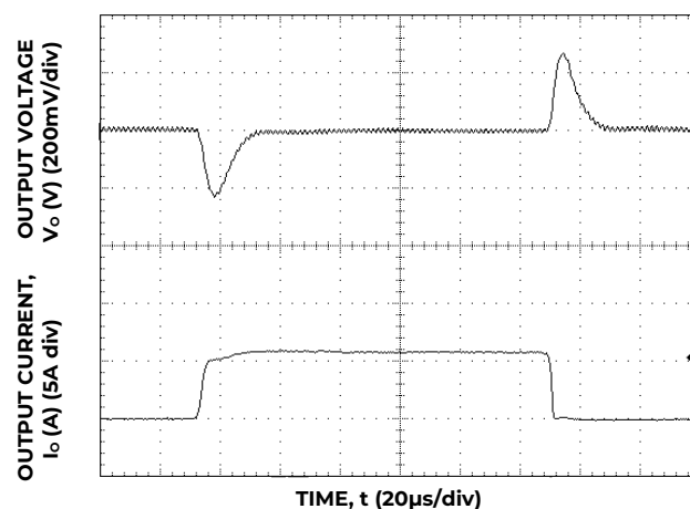
Figure 22. Transient Response to Dynamic Load Change from 0% to 50% to 0% with V IN =5V.
