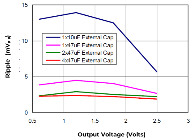
Figure 37. Output ripple voltage for various output voltages with external 1x10 µF, 1x47 µF, 2x47 µF or 4x47 µF ceramic capacitors at the output (12A load). Input voltage is 3.3V.
