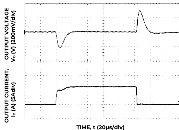
Figure 10. Transient Response to Dynamic Load Change from 0% to 50% to 0% with V IN =5V.
