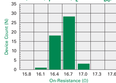
Form-A Typical On-Resistance Distribution (N = 50, I_F = 5 mA, I_L = 120 mA DC )
