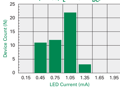
Form-A Typical I_F for Switch Dropout (N = 50, I_L = 120 mA DC )
