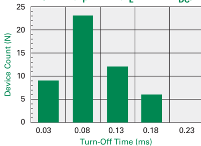
Form-A Typical Turn-Off Time (N = 50, I_F = 5 mA, I_L = 120 mA DC )
