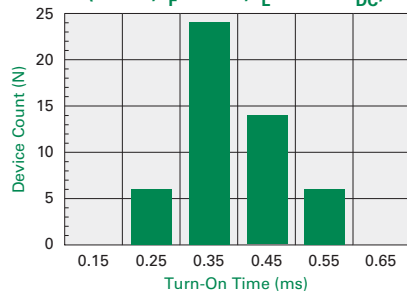
Form-A Typical Turn-On Time (N = 50, I_F = 5 mA, I_L = 120 mA DC )
