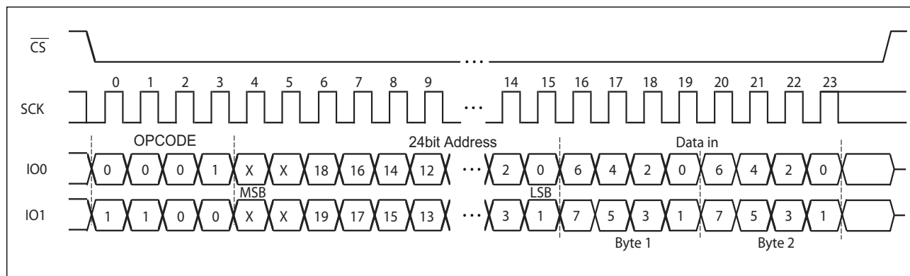
WDAD Command Sequence (DPI mode)
