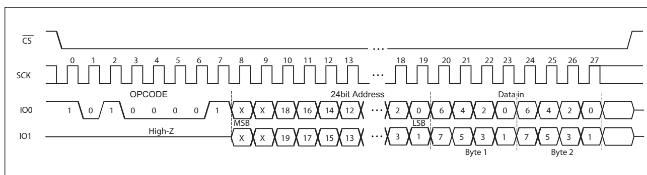
WDAD Command Sequence
