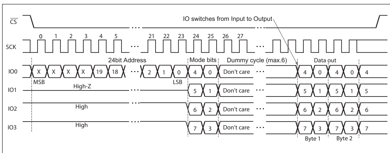
FRQO Command Sequence (XIP mode)
