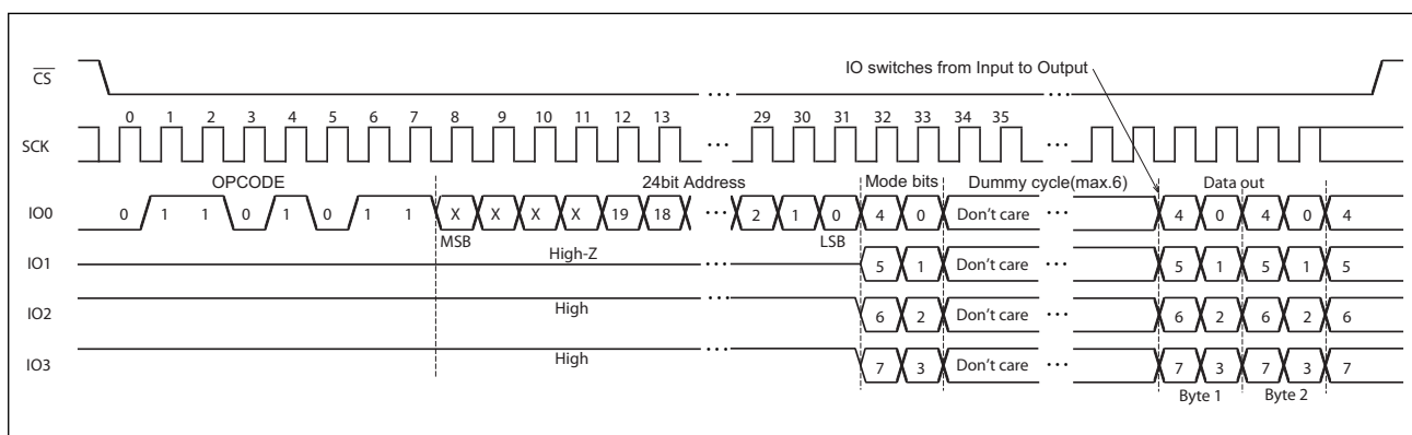
FRQO Command Sequence
