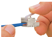
Inserting a conductor via operating lever.
