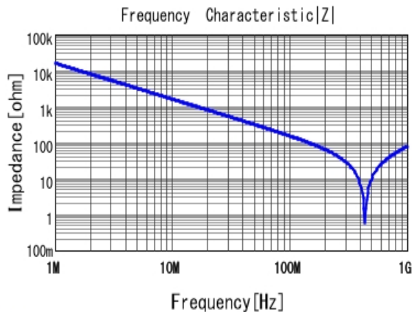
■ DE11XRA100KJ4BP01F |Z| DC0V, 20degC
