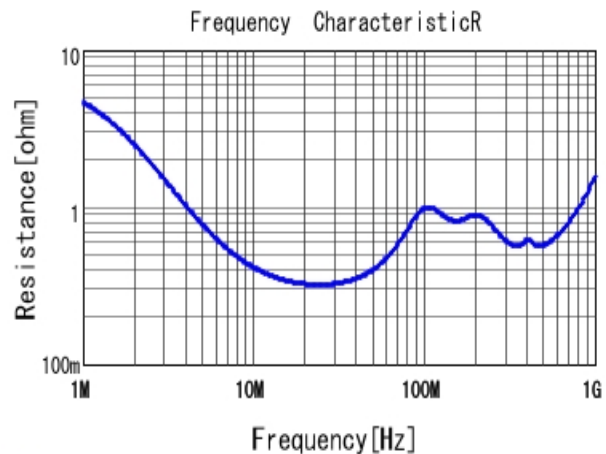
■ DE11XRA100KJ4BP01F R DC0V, 20degC
