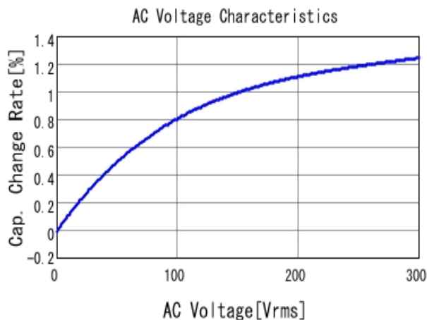
■ DE11XRA100KJ4BP01F C-AC Voltage capchange, DC0V, 20.0
