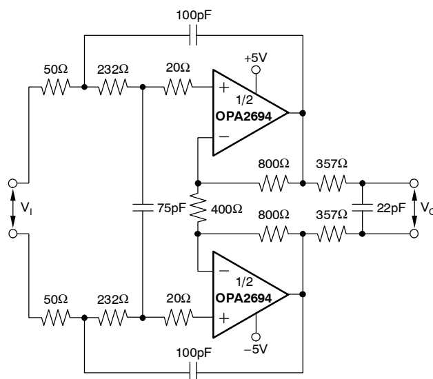
Low-Power, Differential I/O, 3rd-Order Butterworth Active Filter
