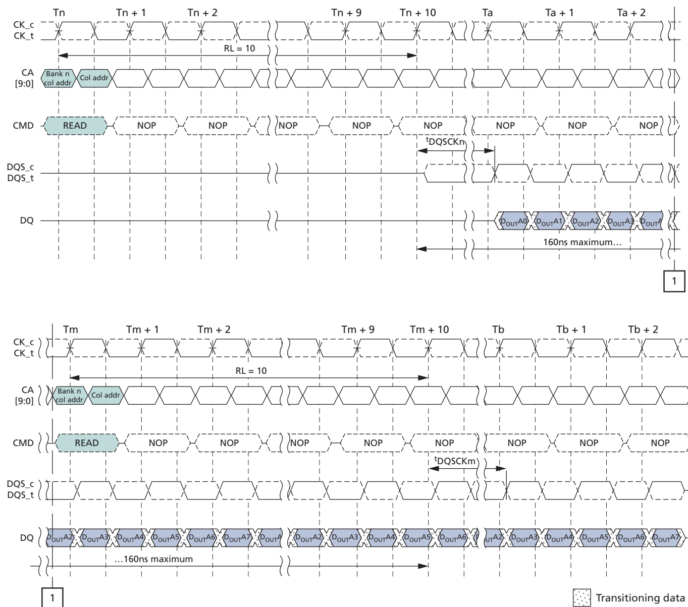
Figure 22: t_{DQSKDS} Timing
