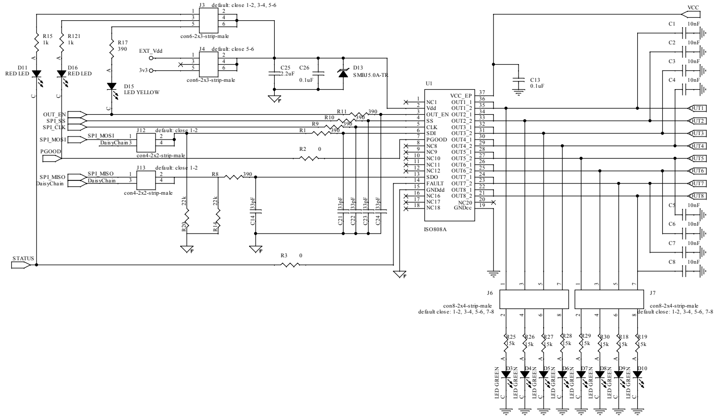
Figure 2. X-NUCLEO-OUT12A1 circuit schematic (2 of 2)
