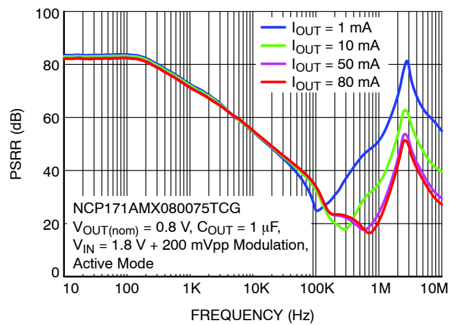
Figure 51. PSRR vs. Frequency in Active Mode
